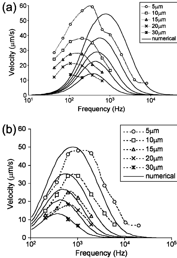
FIG. 9. Comparison of the calculated horizontal electro-osmotic velocity at the surface of the electrodes and the experimental measurements of the fluid velocity across the electrode surface. The data are plotted as a function of frequency (in Hz) for several positions on the electrodes and for electrolyte A (a) and electrolyte B (b). The impedance of the double layer was given by Z_{DL} = \lambda_D / (i\omega\epsilon) and the amplitude of applied voltage was 0.5 V.
