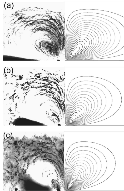
FIG. 12. Comparison of the numerically computed streamlines for 500 \mu\text{m} wide electrodes and the experimental streamlines for the three frequencies used in the experimental observations: (a) 100, (b) 300, and (c) 1000 Hz. The experimental images have been inverted.
